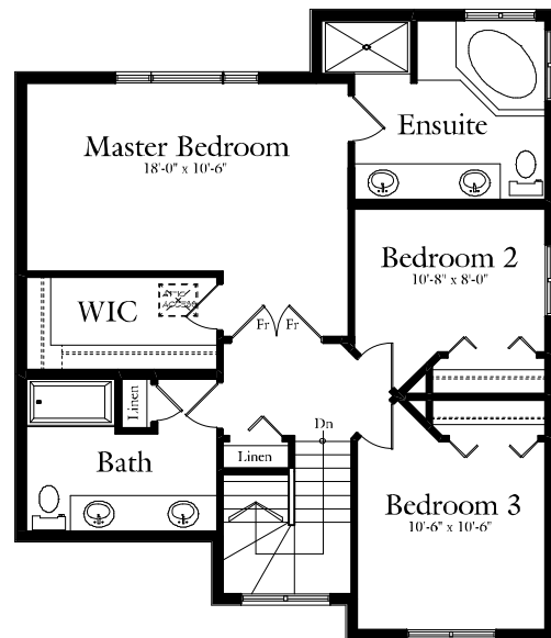
Second Floor Plan 860 SQ.FT.
