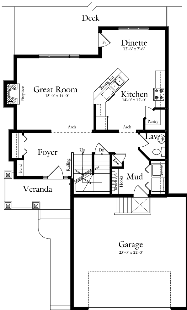
Main Floor Plan 877 SQ.FT.
